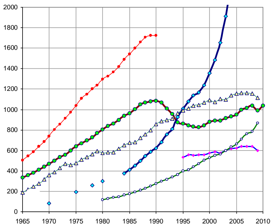
Производство электроэнергии, млрд. кВт-ч. Источники: National Bureau of Statistics of China; Japan Statistical Yearbook, 2008; Statistical Handbook of Japan 2008; United Nations Statistics Division, UN Industrial Commodity Statistics Database; Eurostat; EIA; BP Statistical Review of World Energy; Росстат, Госкомстат.
